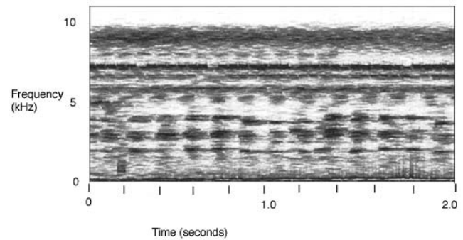
Figure 1. Sonagram of calls of Calayan Rail, Longog, Calayan island, Philippines, May 2004.
